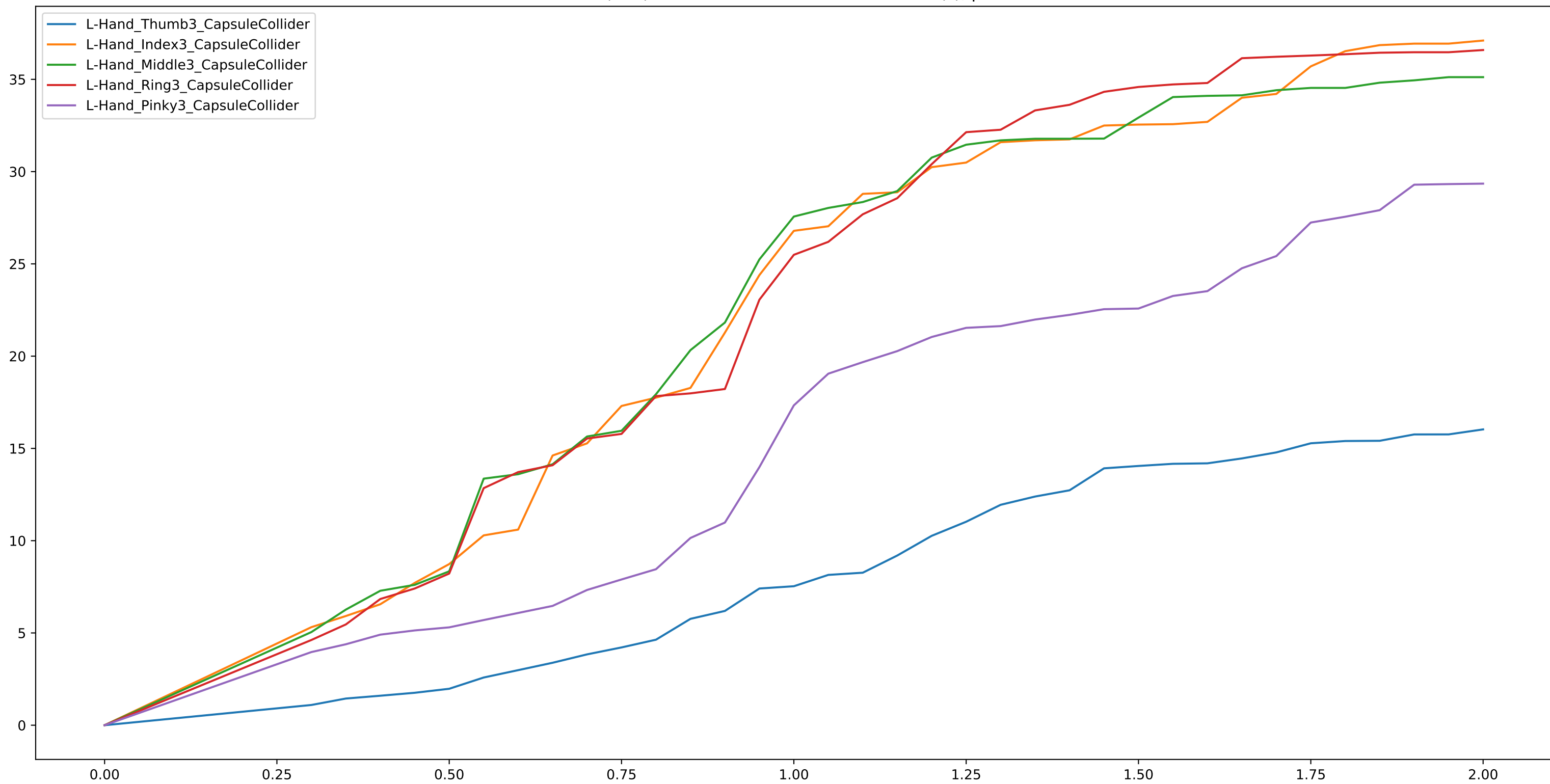
Tolerance (mm) function of Time Prediction Known (s), per Phalanx
