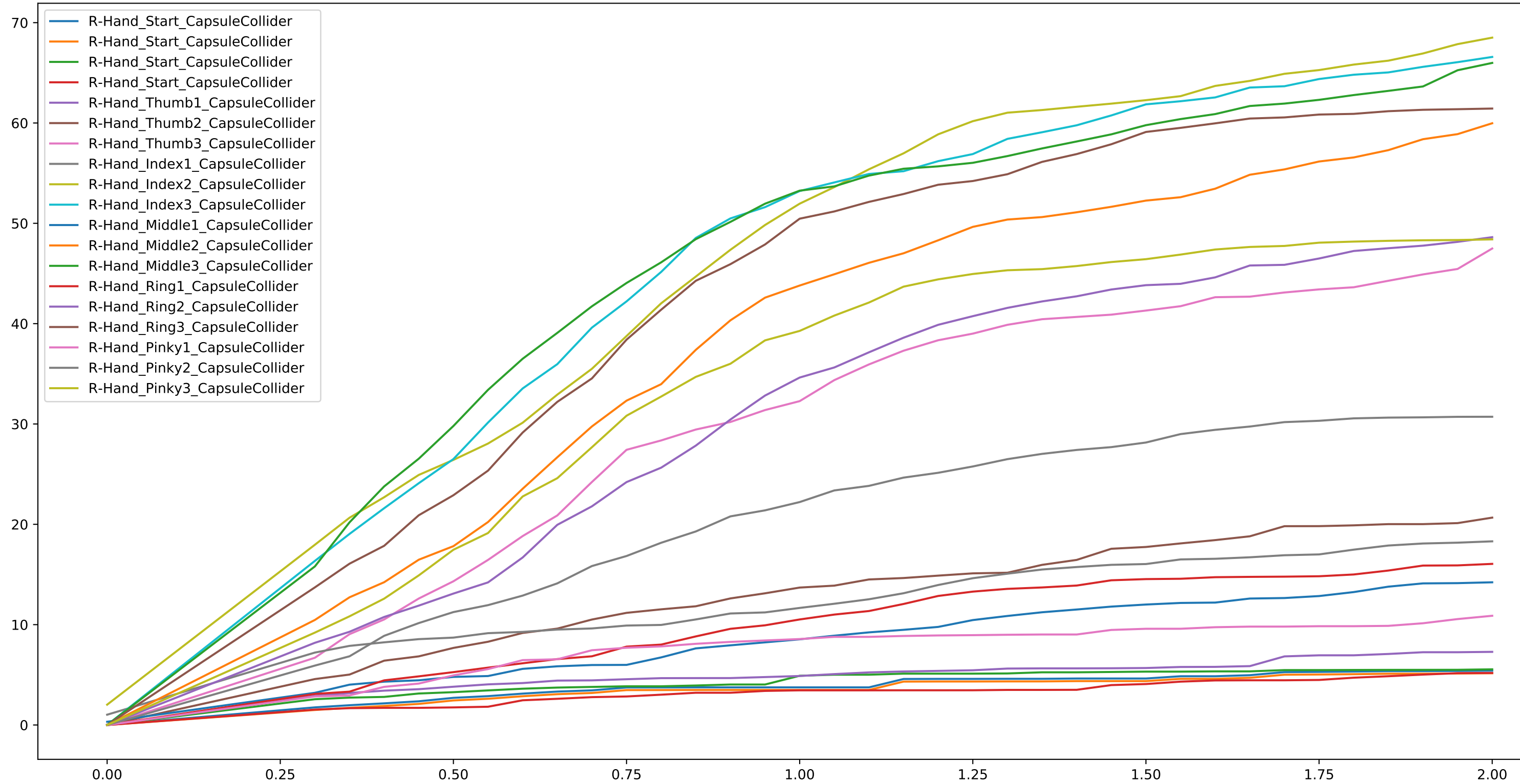
Tolerance (mm) function of Time Prediction Known (s), per Phalanx
